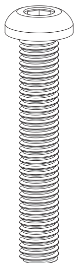
A M10x60
